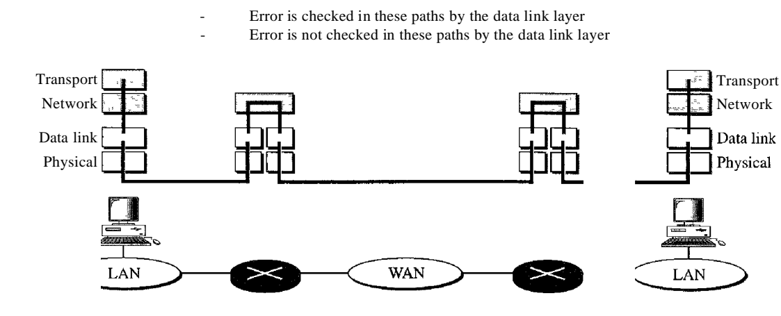
Figure 23.7 Error control
