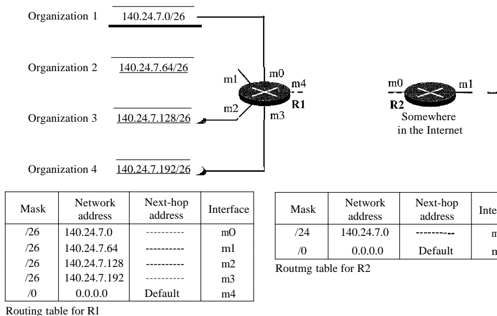
Figure 22.7 Address aggregation
