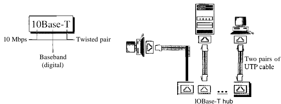
Figure 13.12 10Base-T implementation
