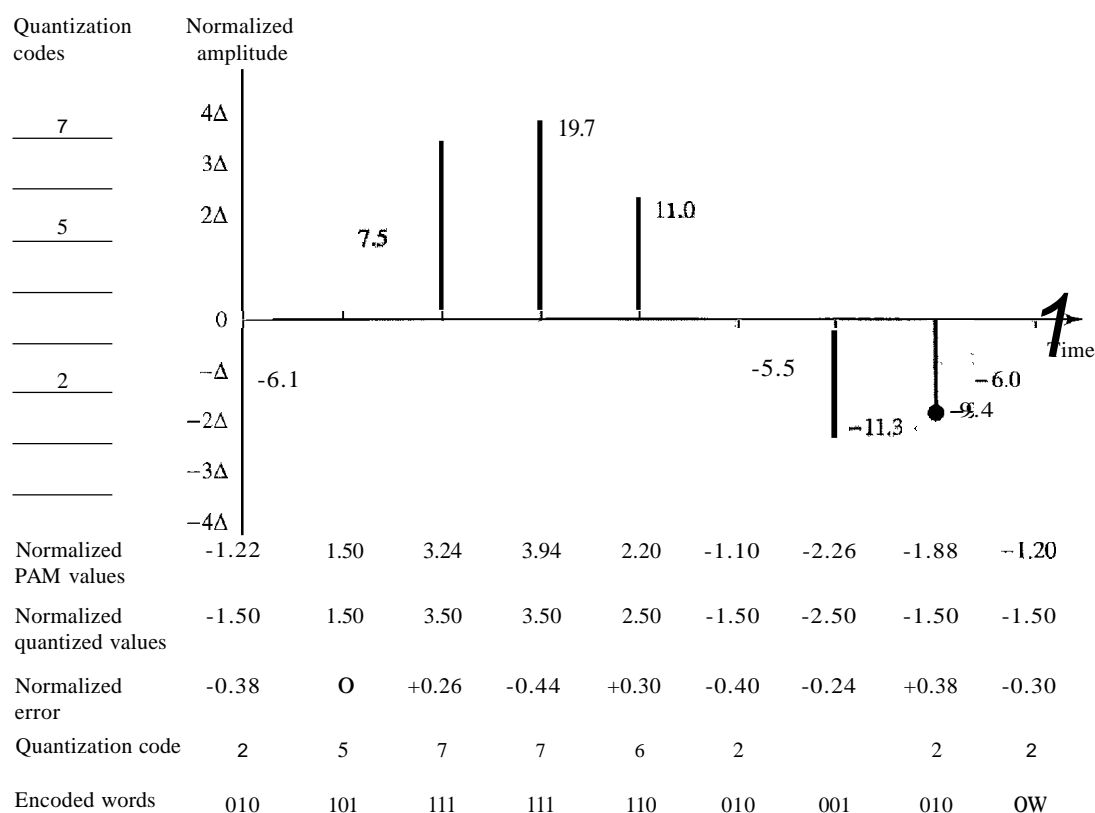
Figure 4.26 Quantization and encoding of a sampled signal
