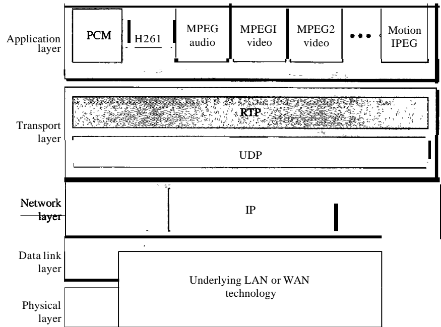
Figure 29.18 RTP
