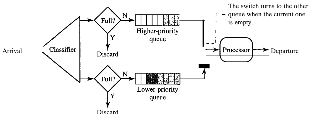
Figure 24.17 Priority queuing
