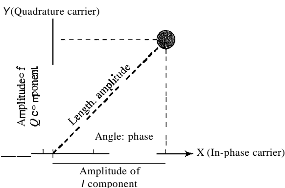
Figure 5.12 Concept of a constellation diagram
