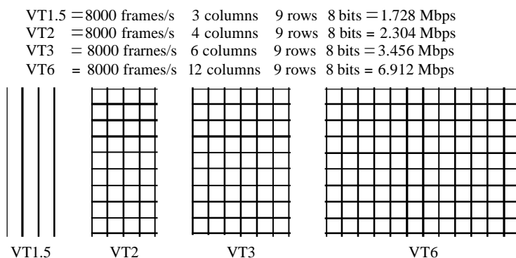
Figure 17.26 Virtual tributary types
