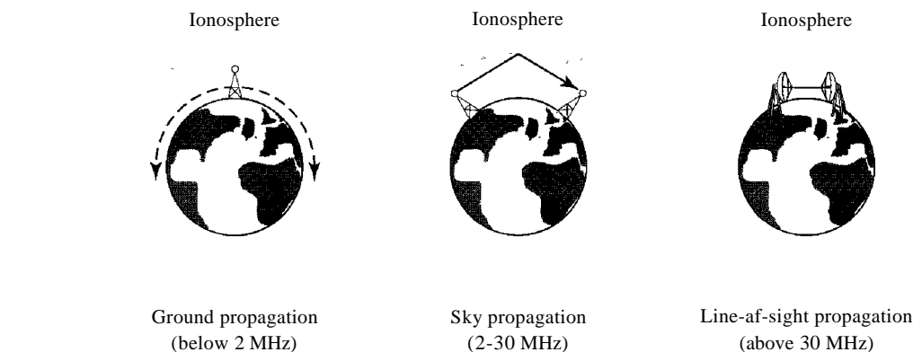
Figure 7.18 Propagation methods
