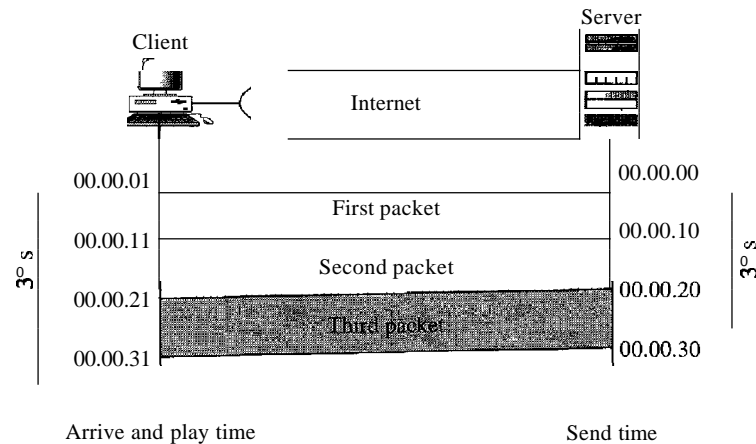
Figure 29.14 Time relationship
