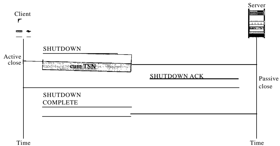
Figure 23.35 Association termination
