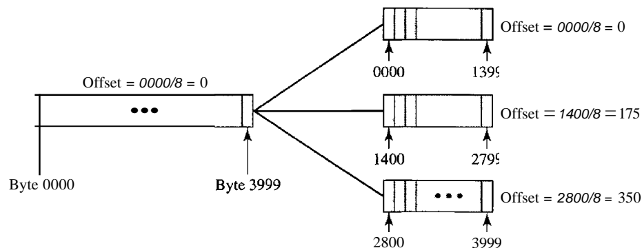
Figure 20.11 Fragmentation example
