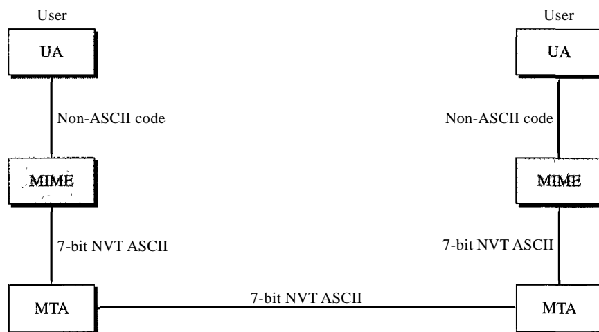
Figure 26.14 MIME
