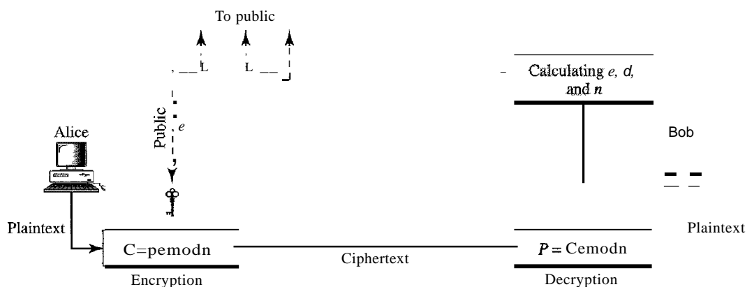
Figure 30.24 RSA
