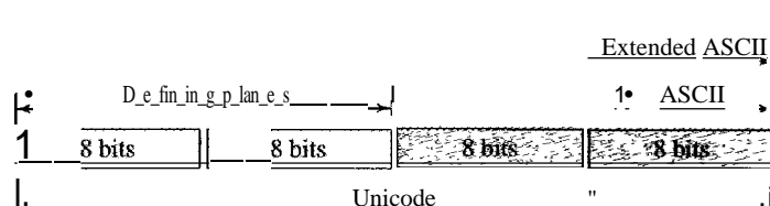
Figure A.I Unicode compatibility
