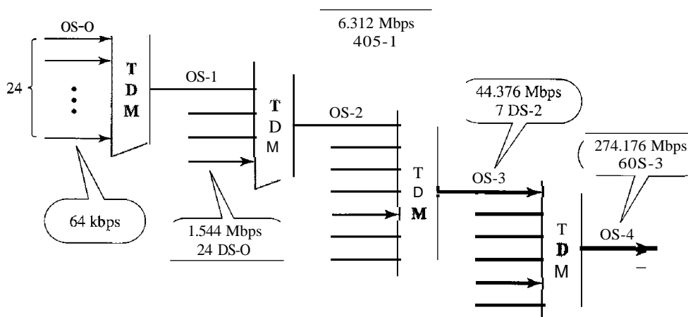
Figure 6.23 Digital hierarchy
