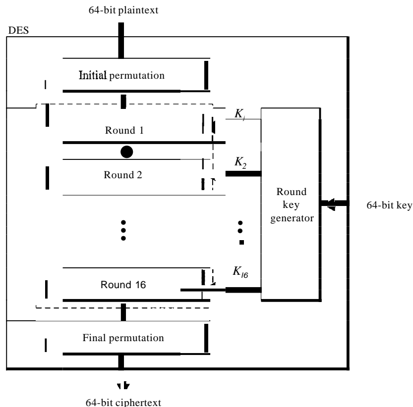
Figure 30.13 DES
