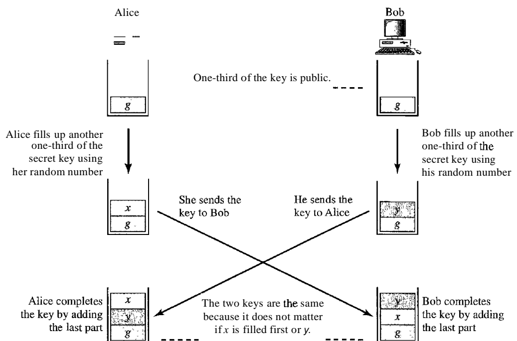
Figure 30.27 Diffie-Hellman idea
