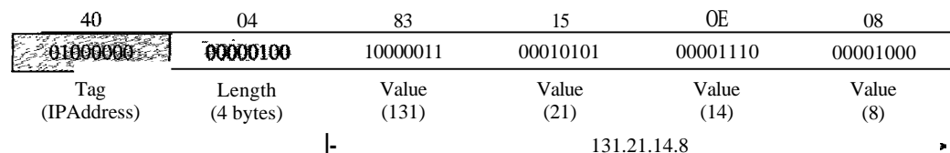
Figure 28.14 Example 28.4, IPAddress 131.21.14.8
