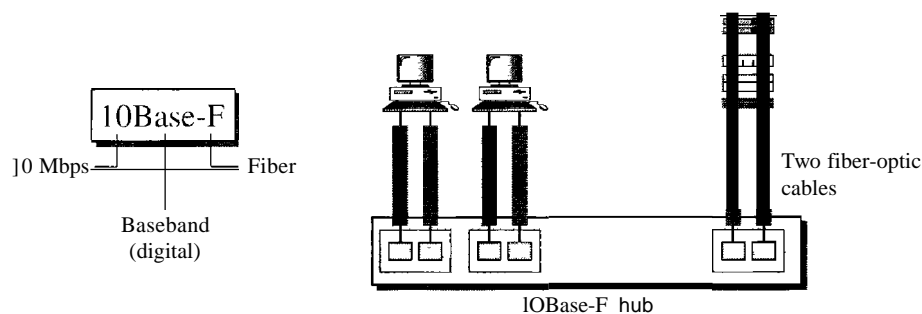
Figure 13.13 10Base-F implementation
