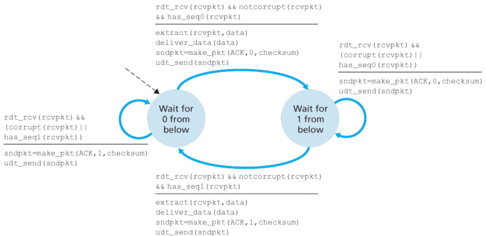
Figure 3.14 rdt2.2 receiver
