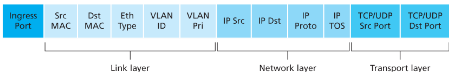
Figure 4.29 Packet matching fields, OpenFlow 1.0 flow table
