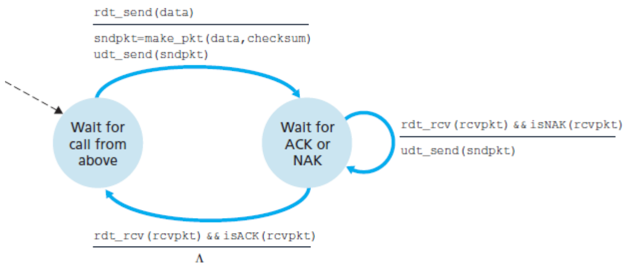
Figure 3.10 rdt2.0 – A protocol for a channel with bit errors
