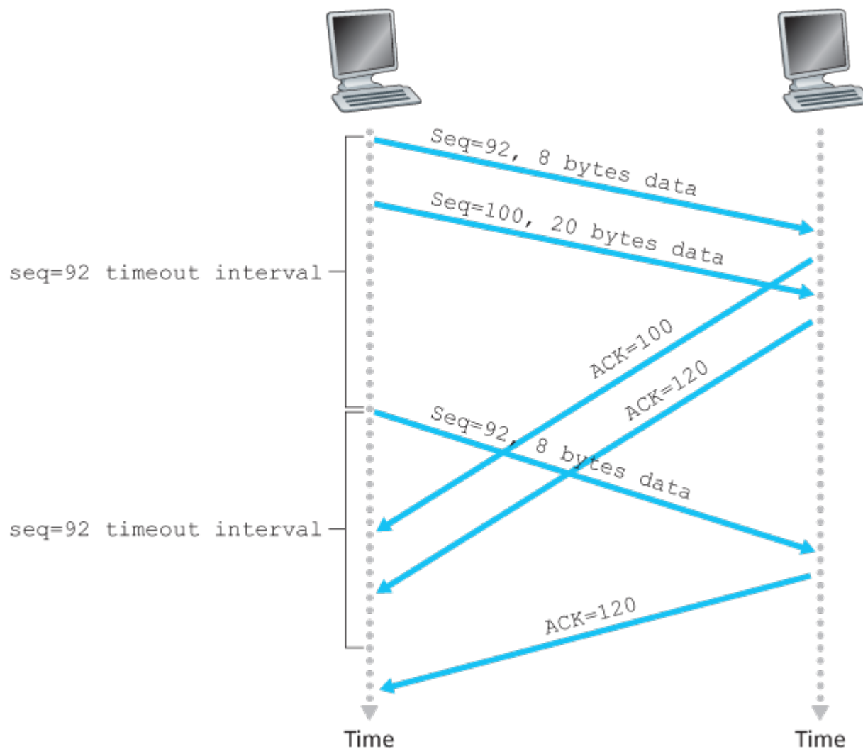
Figure 3.35 Segment 100 not retransmitted
