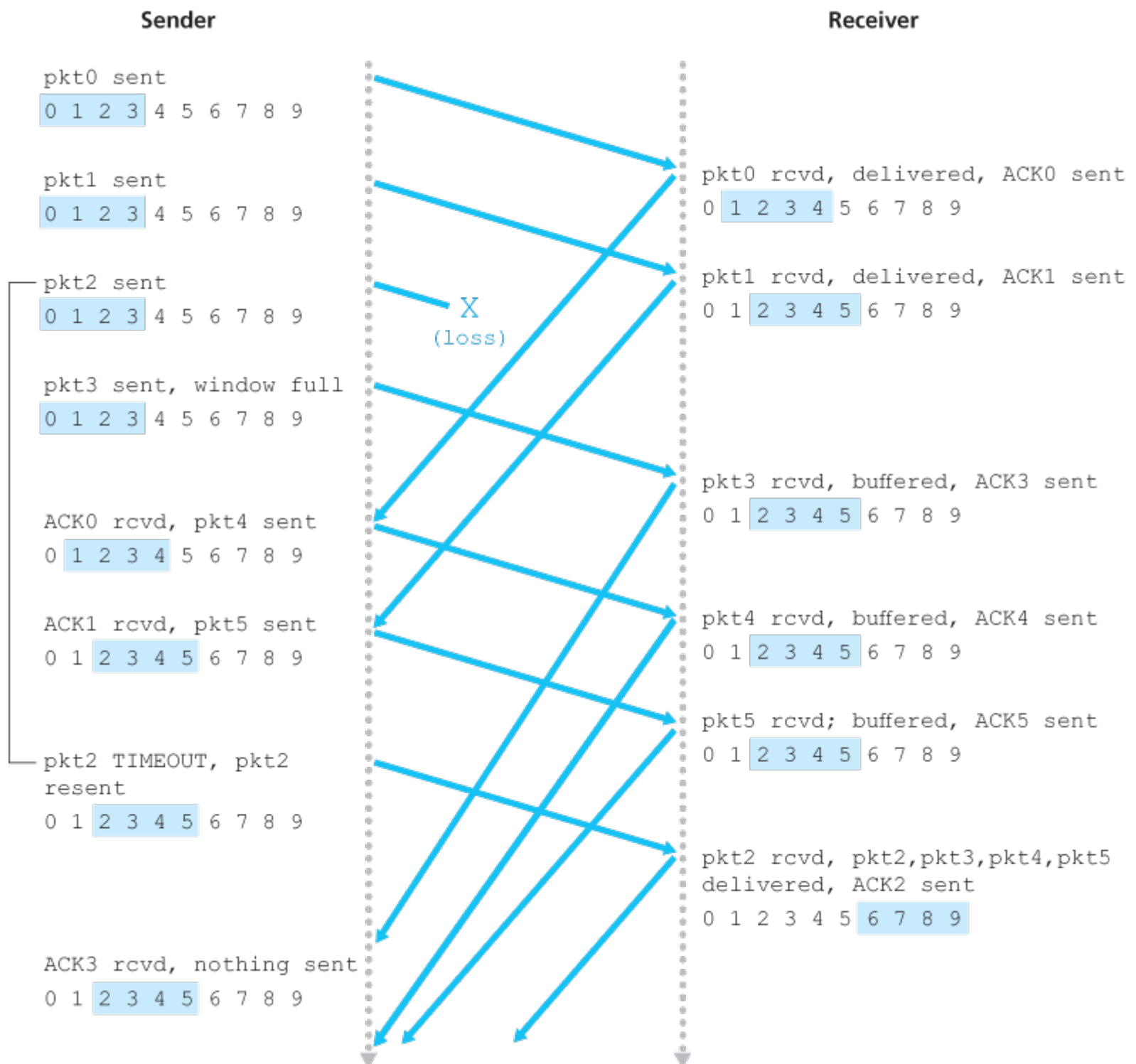
Figure 3.26 SR operation
