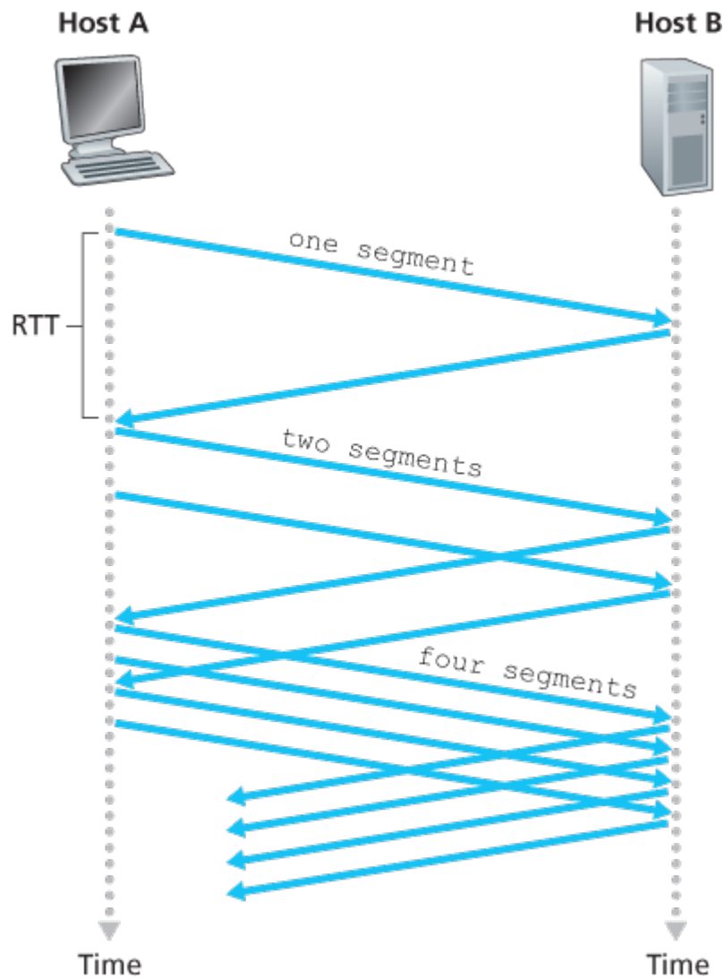
Figure 3.50 TCP slow start
