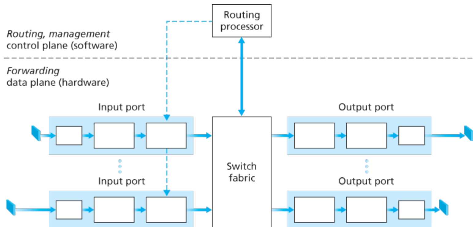
Figure 4.4 Router architecture
