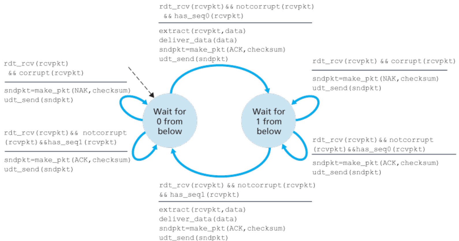
Figure 3.12 rdt2.1 receiver
