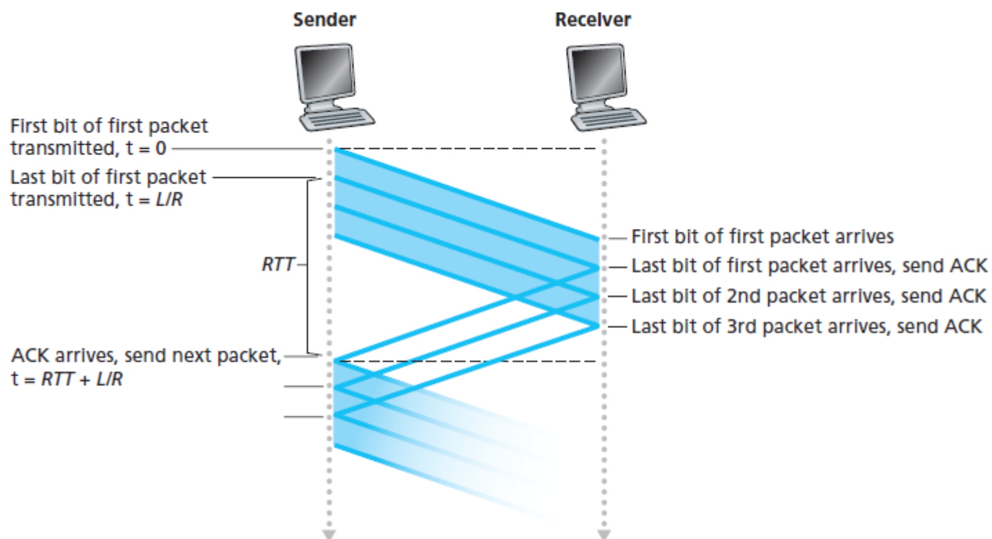
b. Pipelined operation
